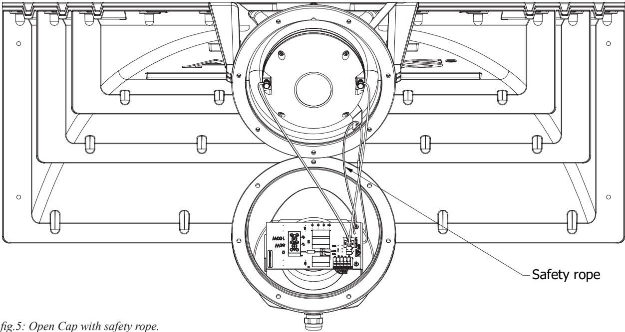
fig.5: Open Cap with safety rope.
