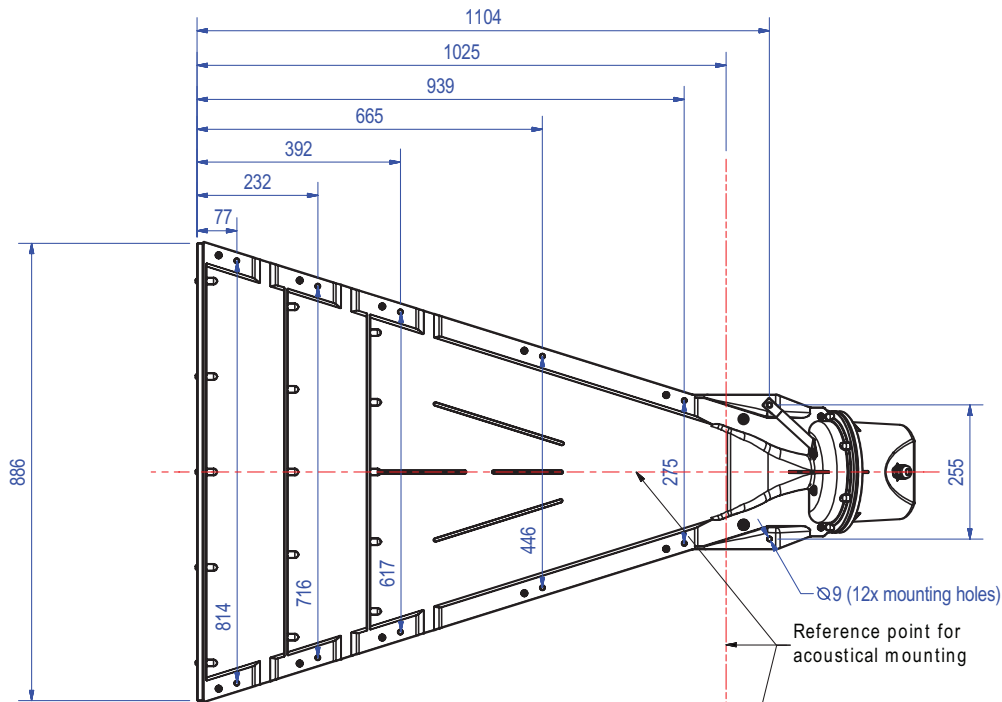
fig.2: Mechanical references.
