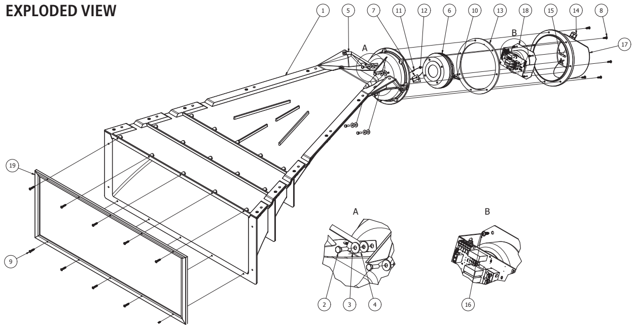
fig. 4: Exploded View.
